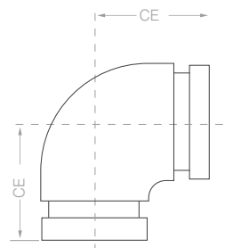
SDG-105 90° Short Radius Elbow
