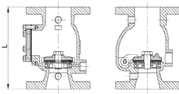
Flange x Flange, SD-AVA-300F
