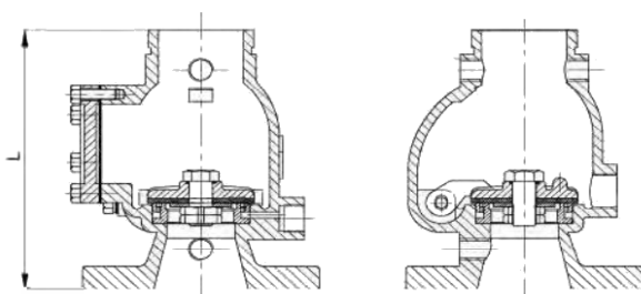
Groove x Flange, SD-AVA-300FGB
