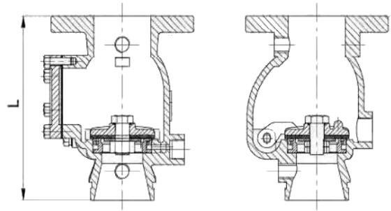
Flange x Groove, SD-AVA-300FGA
