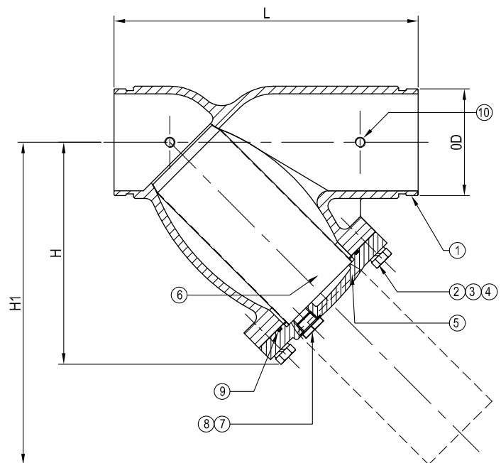
SECTIONAL FRONT VIEW
