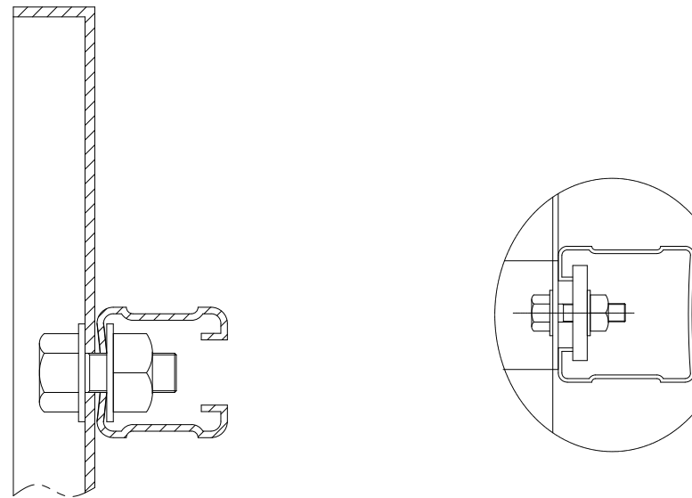
(MOUNTING DETAIL B/W BASE PLATE& MOUNTING RAIL)
