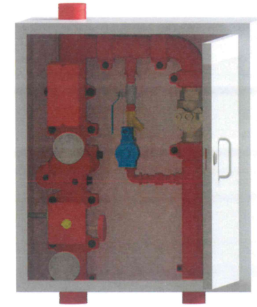
VIEW- A
