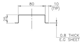
DETAIL - T
